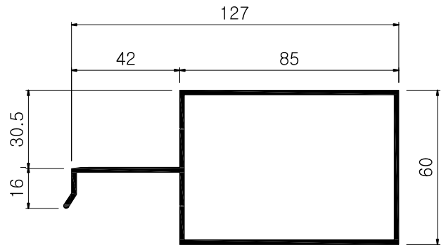
K A T - 2 2 0 3 2.38 kg/m, 1.8T
