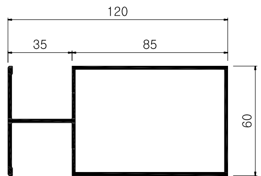
K A T - 2 2 0 5 1.88 kg/m, 1.8T
