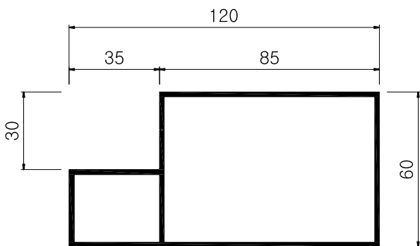
K A T - 2 2 0 6 1.87 kg/m, 1.8T
