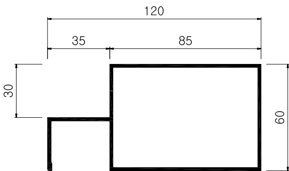
K A T - 2 2 0 4 1.72 kg/m, 1.8T
