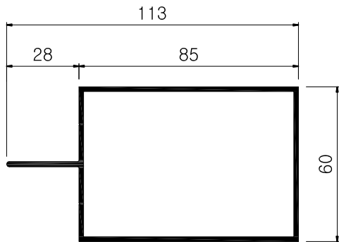
K A T - 2 2 0 2 1.52 kg/m, 1.8T
